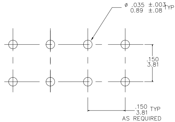
FIG.1 SCALE 5/1
