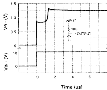
Time ( \mu s ) Transient Response ( I_R = 5mA )
