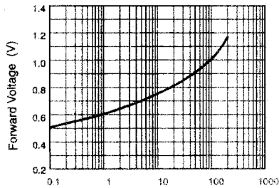
Forward Current (mA) Forward Characteristics
