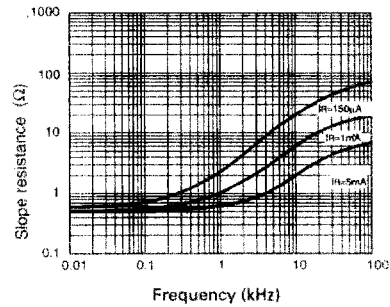
Frequency (kHz) Slope Resistance v Frequency
