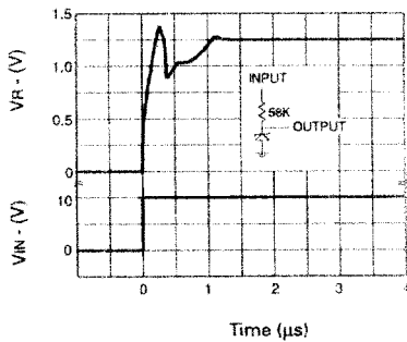
Time ( \mu s ) Transient Response ( I_R = 150\mu A )
