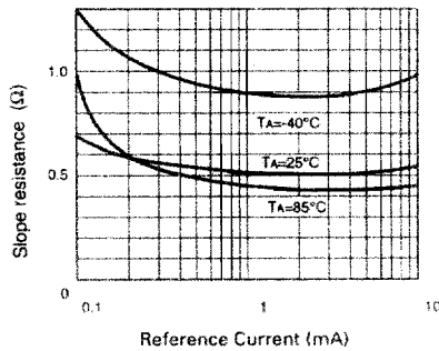
Reference Current (mA) Slope Resistance v Current
