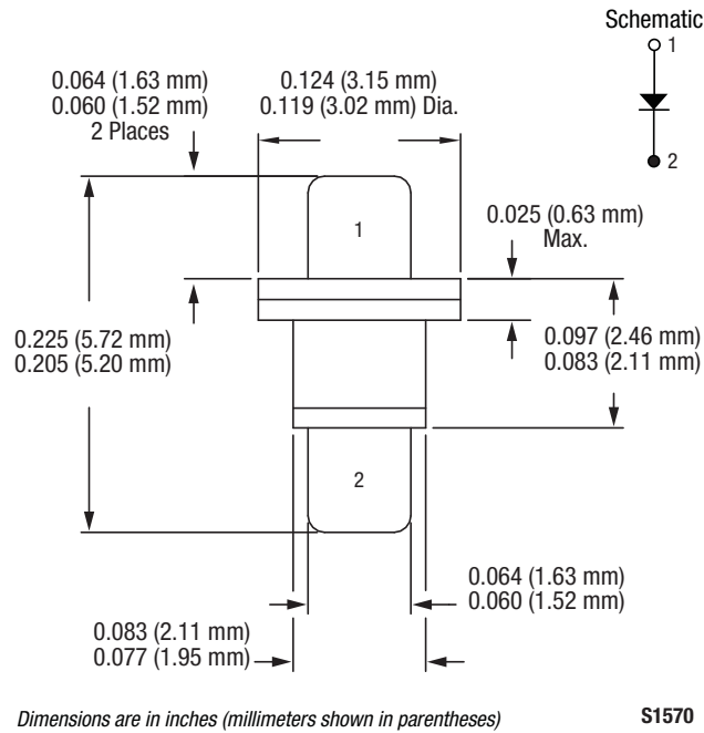
Figure 8. -210 Package
