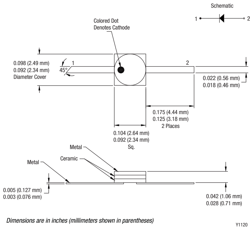
Figure 10. -240 Package
