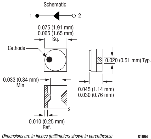
Figure 9. -219 Package
