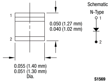
Figure 7. -203 Package
