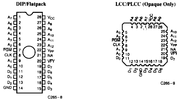
Figure 1. Programming Pinout
