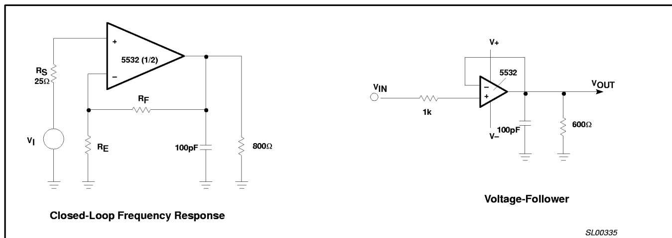
Figure 4. Test Circuits
