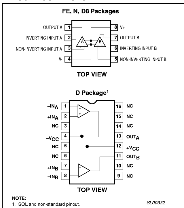
Figure 1. Pin Configurations
