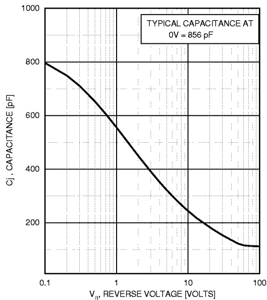
Fig.3 Typical Capacitance
