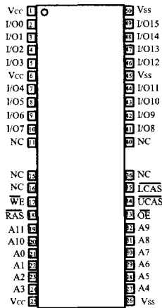
44(50)TSOP II
