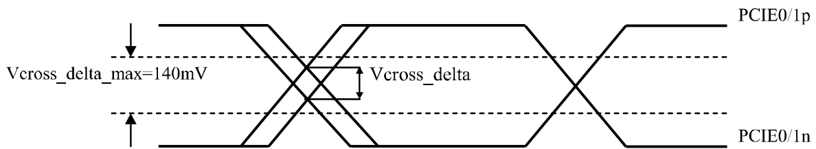
Figure 5. Definition of Output Cross Point Voltage Deviation
