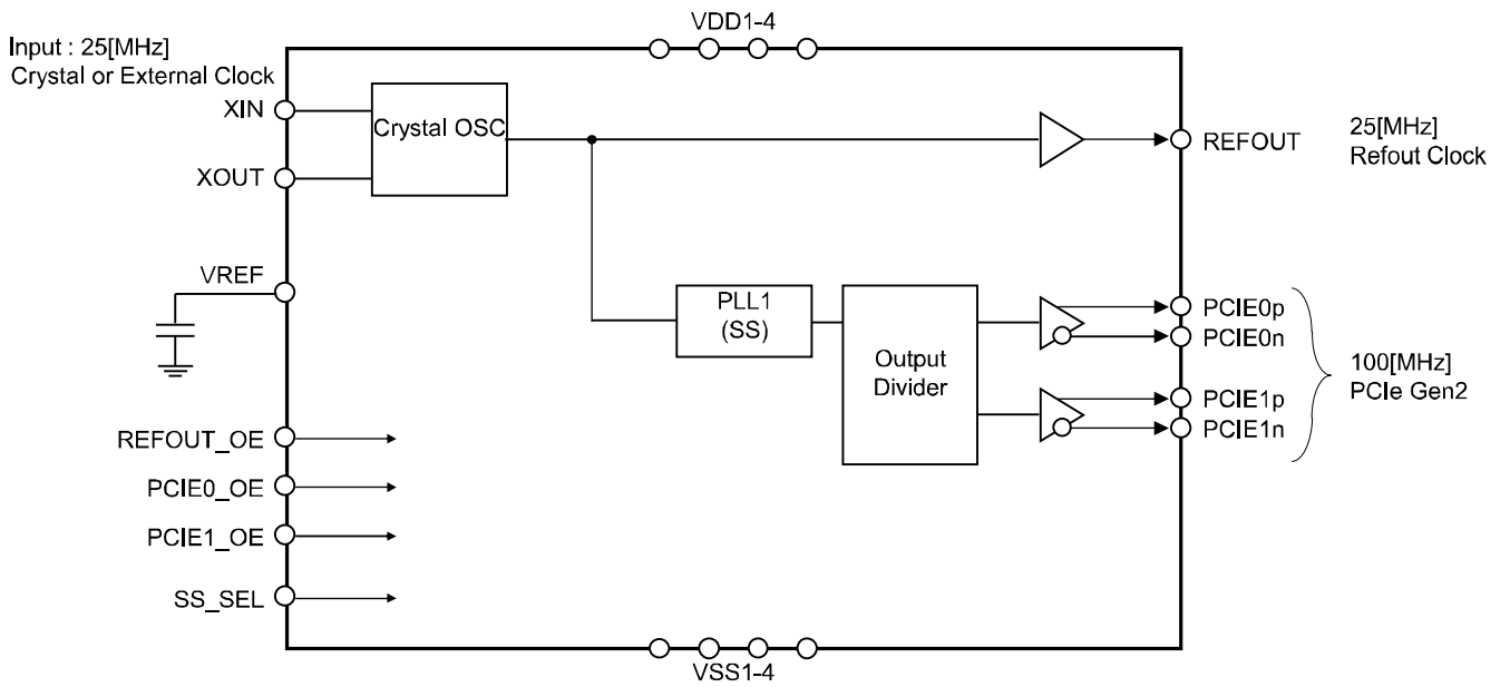
Figure 1. AK8160BV2 Block Diagram
