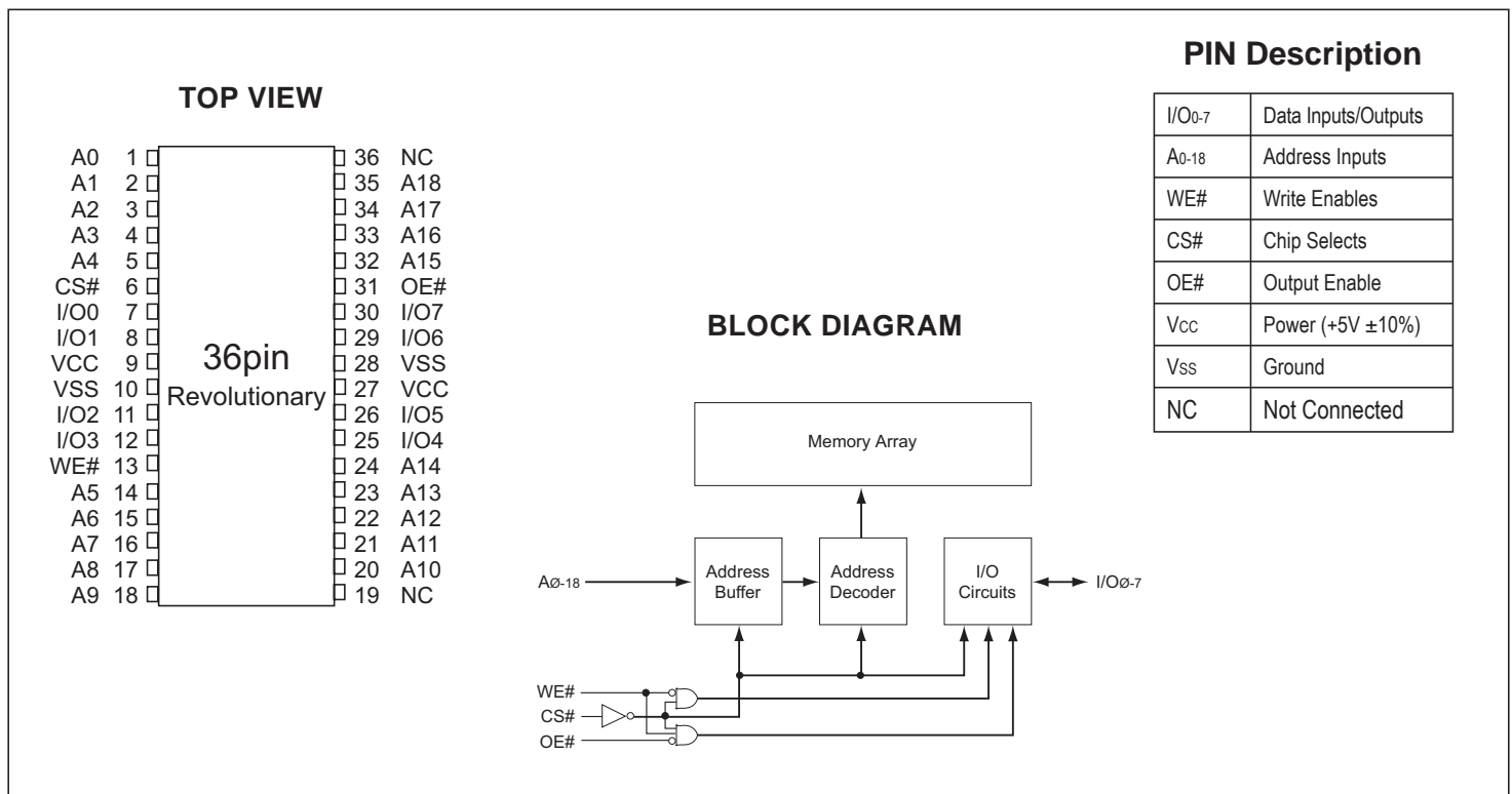
FIG. 1 – PIN CONFIGURATION
