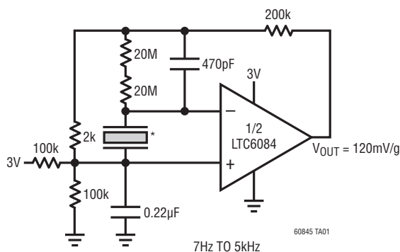
Shock Sensor Amplifier
