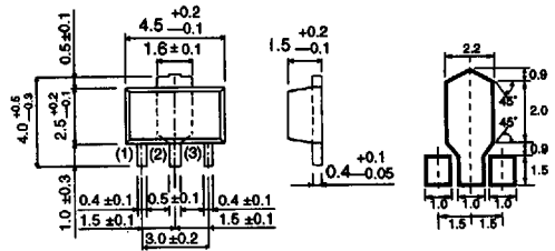
2SB1427 (MPT3)
