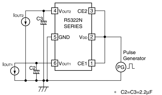
Fig.3 Ripple Rejection, Line Transient Response Test Circuit
