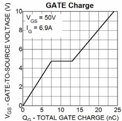
Figure 5. GATE Charge
