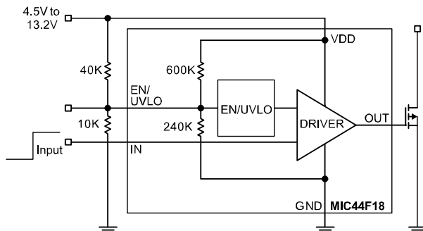
MOSFET Driver with 6.2V Programmed UVLO Internally Set
