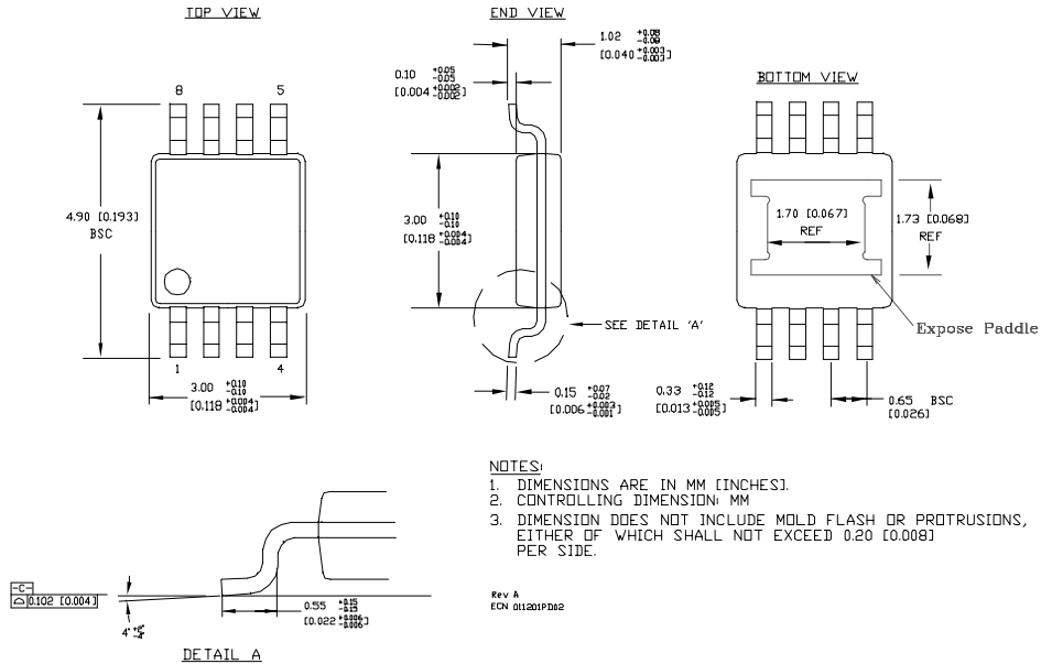
8-Pin ePad MSOP (M)
