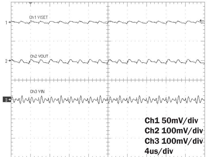
Spotlight Mode Ripple, R ISET = 1.25Ω
