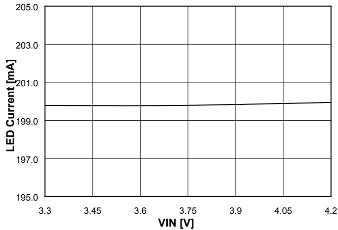
Flash Current at 100ms, RISET = 1.25Ω, VOUT = 3.28V
