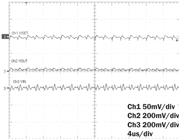
Flash Mode Ripple, R ISET = 1.25Ω
