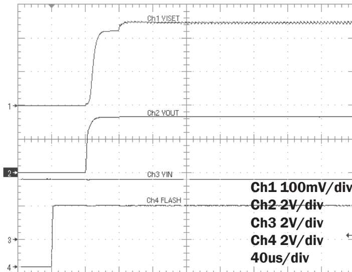
Startup Flash Mode 200mA
