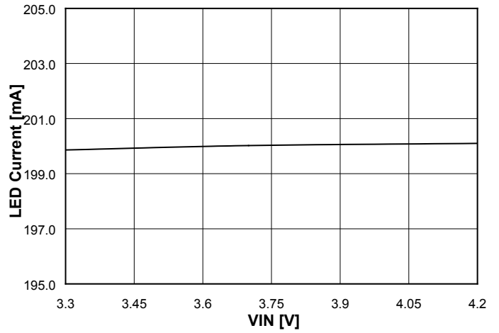
Flash Current at 10ms, RISET = 1.25Ω, VOUT = 3.30V
