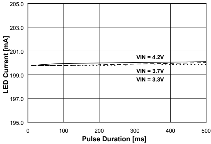
200mA Flash Duration, RISET = 1.25Ω, VOUT = 3.30V(start) to 3.25V(LED heated 500ms)
