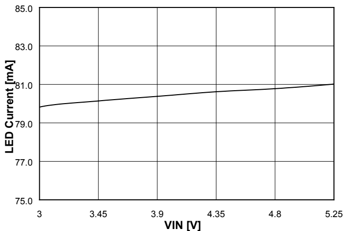
80mA Spotlight Current, RISET = 1.25Ω, VOUT = 2.96V
