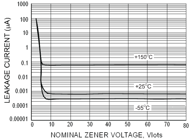
FIG. 7-TYPICAL LEAKGE CURRENT
