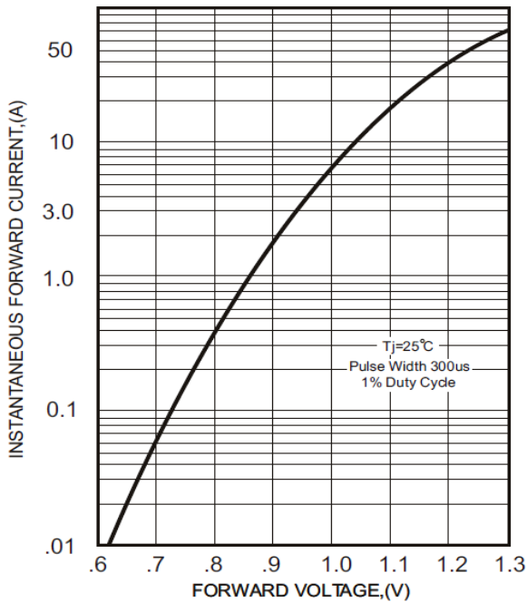
FIG.1-TYPICAL FORWARD CHARACTERISTICS
