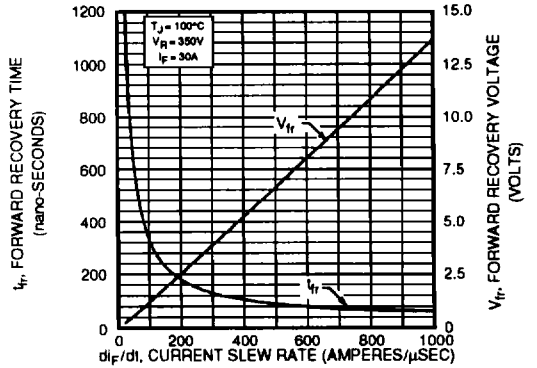
Figure 7, Forward Recovery Voltage/Time vs Current Slew Rate
