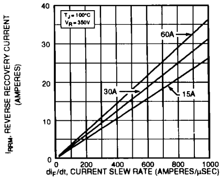
Figure 4, Reverse Recovery Current vs Current Slew Rate
