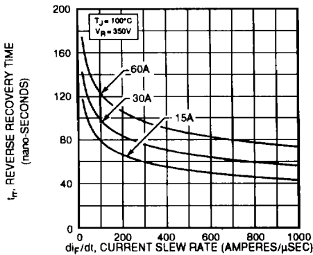
Figure 6, Reverse Recovery Time vs Current Slew Rate
