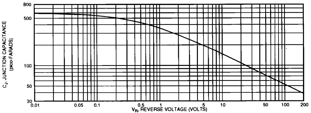
Figure 8, Junction Capacitance vs Reverse Voltage
