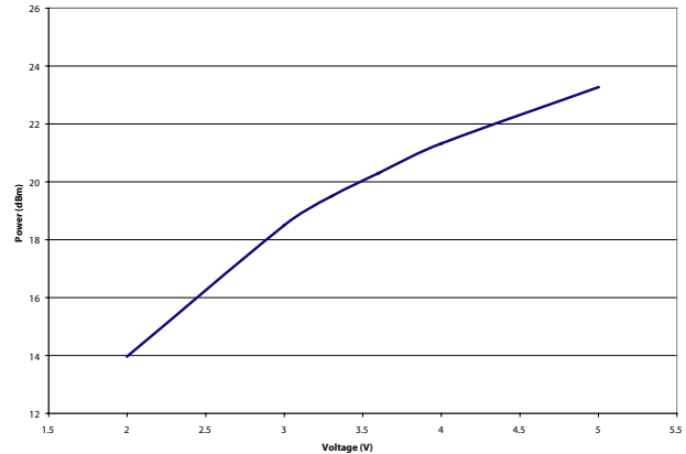
CCMM6004-SC Evaluation board @ 900MHz P1dB Over Voltage
