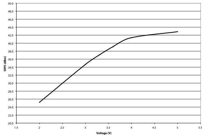
CCMM6004-SC Evaluation board @ 900MHz OIP3 Over Voltage
