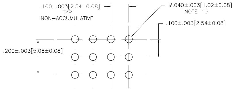
TRIPLE ROW RECOMMENDED HOLE PATTERN SCALE: 4/1
