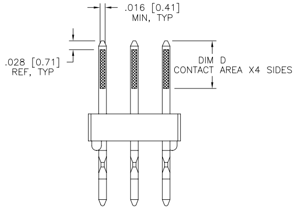
TRIPLE ROW END VIEW
