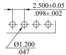
RECOMMENDED HOLE PATTERN
