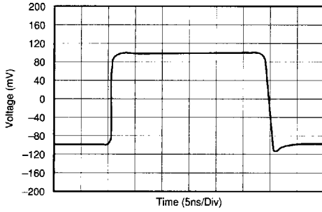
SMALL SIGNAL TRANSIENT RESPONSE ( G = +2 , R_L = 100\Omega )
