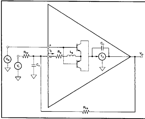
FIGURE 1. Equivalent Circuit.
