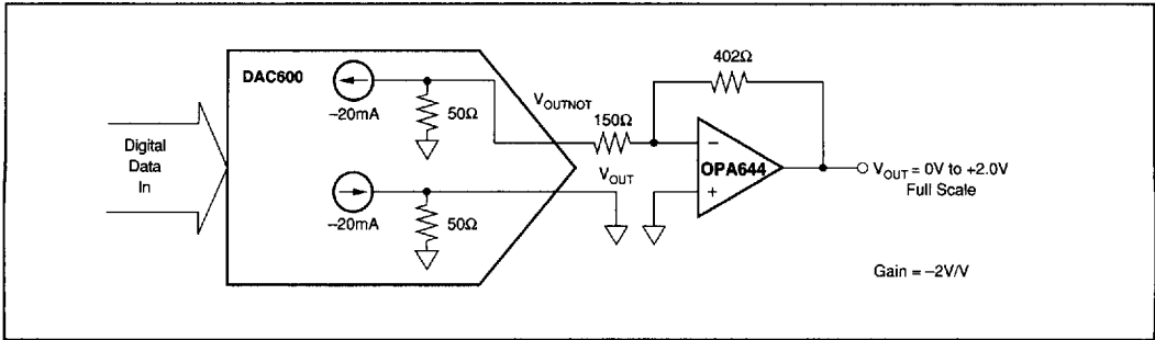
FIGURE 11. Output Amplification for the DAC600.
