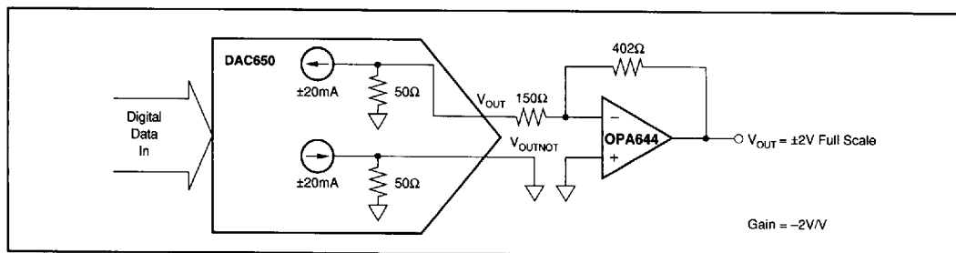
FIGURE 10. Output Amplification for the DAC650.
