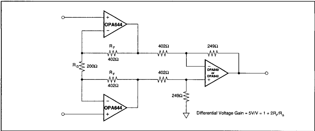
FIGURE 12. Wideband, Fast-Settling Instrumentation Amplifier.
