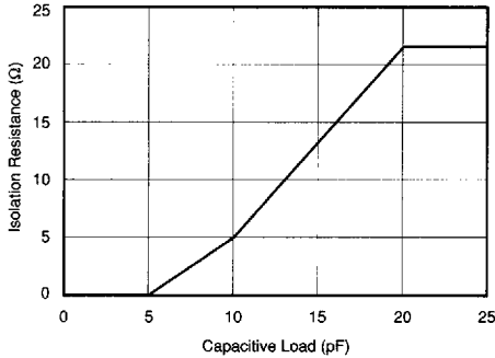
RECOMMENDED ISOLATION RESISTANCE vs CAPACITIVE LOAD
