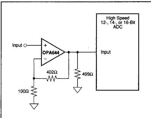
FIGURE 13. Low Distortion Gain Amplifier ( G = +5\text{V/V} ).
