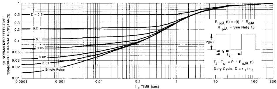
Figure 17. Transient Thermal Response Curve.
