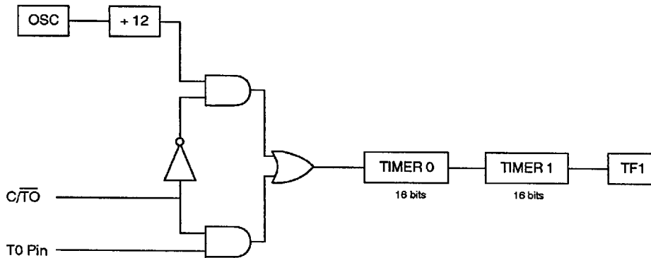
Figure 10.32 Bit Timer/counter.
