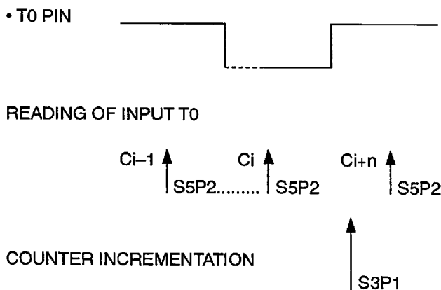
Figure 13. Counter Incrementation Condition.
