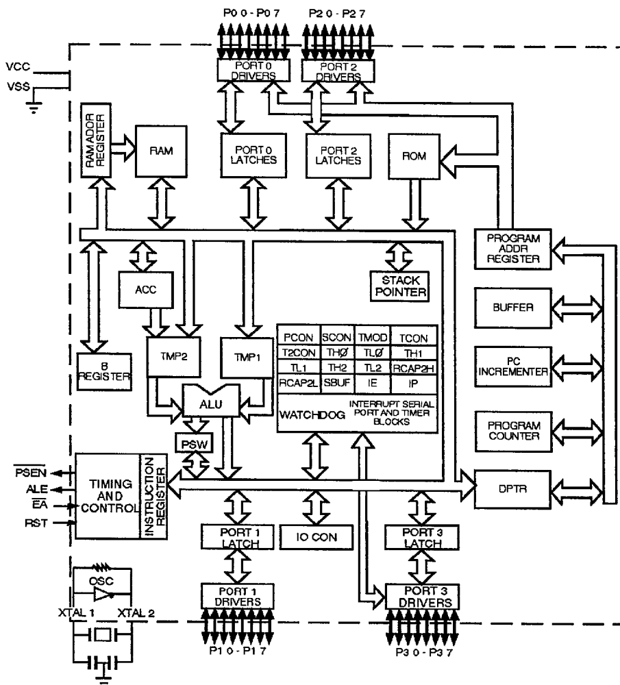
Figure 1. Block Diagram
