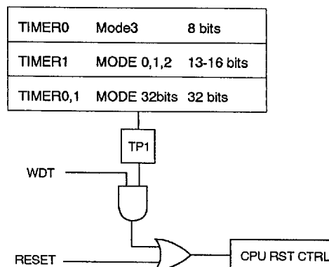
Figure 14. The Different Watchdog Configurations.
