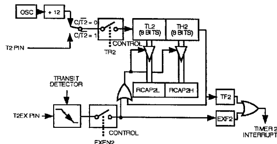
Figure 8. Timer 2 in Auto-Reload Mode.
