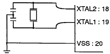
Figure 5. Crystal Oscillator.
