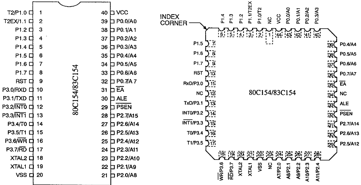
Figure 2. Pin Configuration
