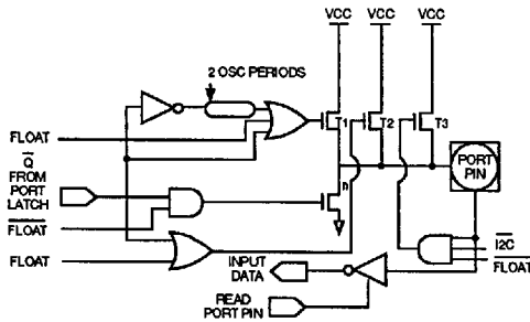
Figure 4. I/O Buffers in the 83C154 (Ports 1, 2, 3).
