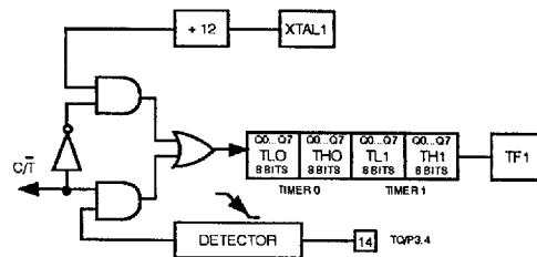
32 bit timer [IOCON bit 6 (T32) = 1]
