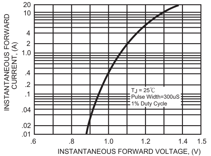
FIG. 2 - MAXIMUM INSTANTANEOUS FORWARD CHARACTERISTICS
