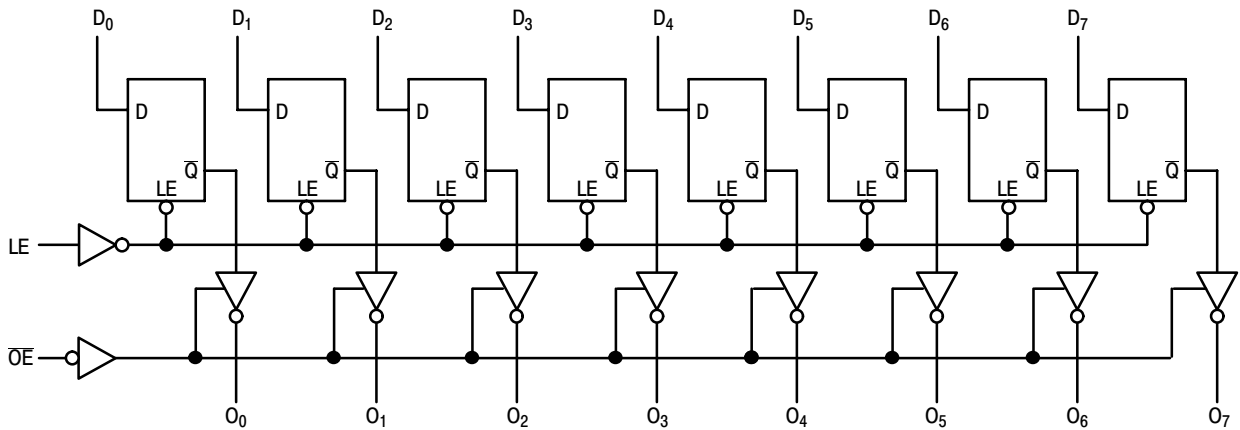
Figure 3. Logic Diagram
