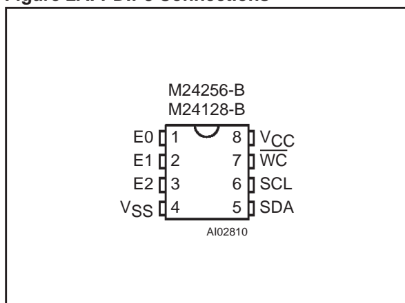
Figure 2A. PDIP8 Connections
