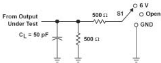
FIGURE 1. LOAD CIRCUIT FOR OUTPUTS
