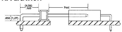
Custom Low Profile Elevated Right Angle Header plugged into Right Angle SSSH Socket
