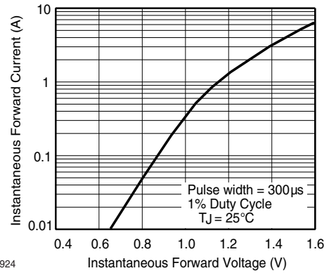
Figure 4. Typical Instantaneous Forward Characteristics for SML4763
