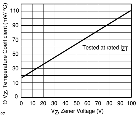
Figure 3. Typical Temperature Coefficients
