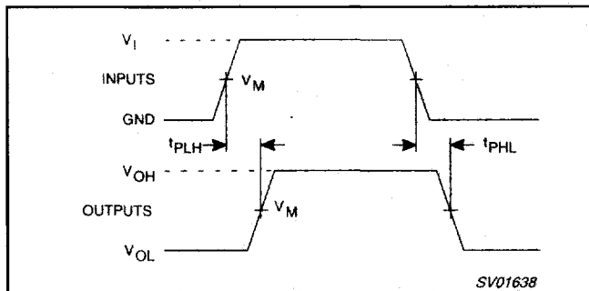
Figure 13. Input ( V_i ) to output ( V_{os} ) propagation delays.
