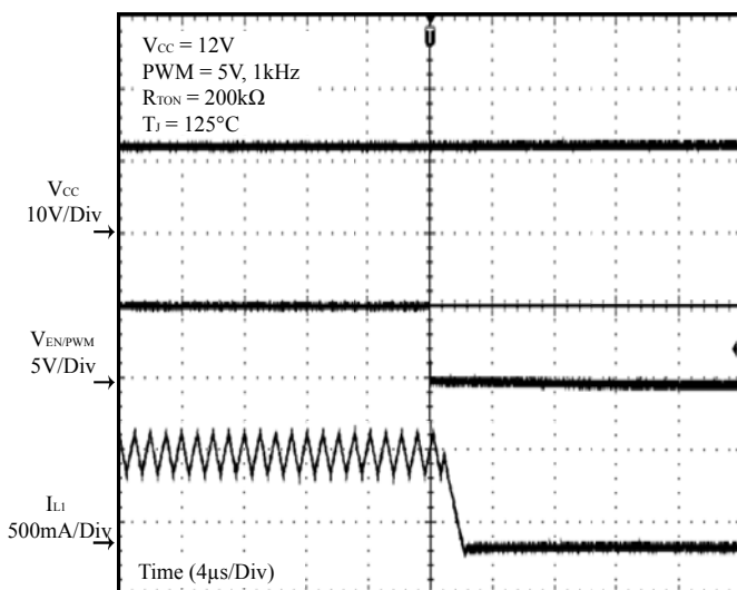
Figure 24 PWM Off
