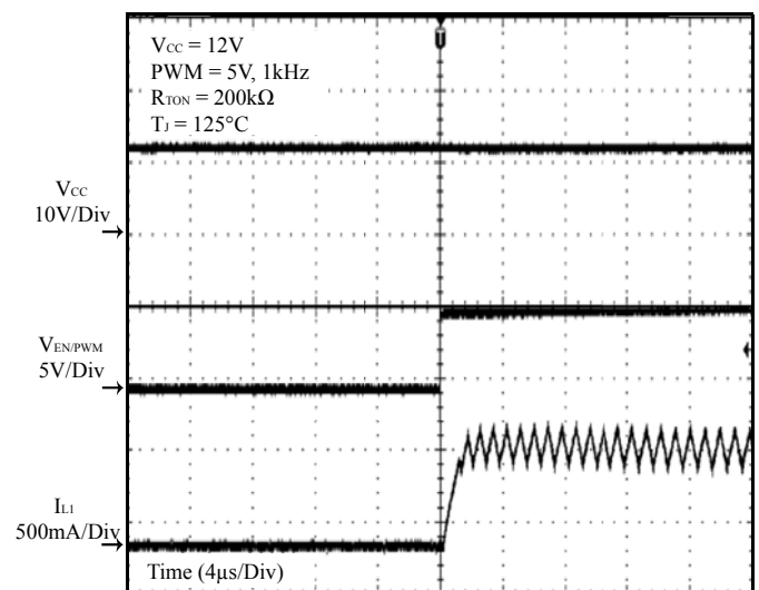
Figure 25 PWM On
