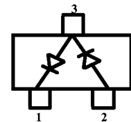
Series Pair
