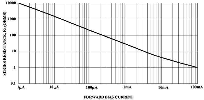
Resistance vs Forward Current (MA4P277 Series)
