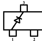
Single
