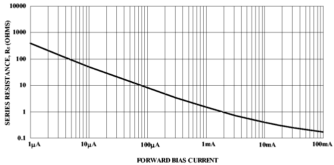
Resistance vs Forward Current (MA4P282 Series)
