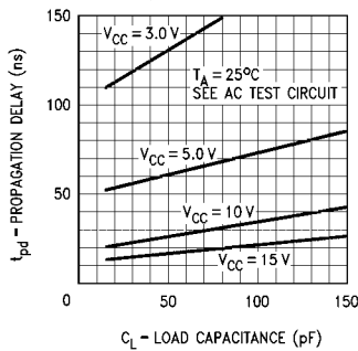
Propagation Delay vs Load Capacitance
