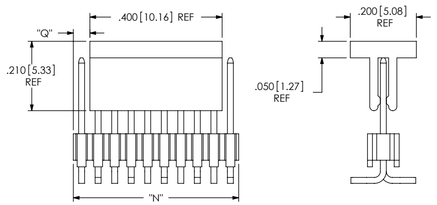
FIG 2 -P: PICK & PLACE "N" = USE MEASURED DIM "Q" = {("N" - .400 [10.16]) / 2} ± .020 [.51]
