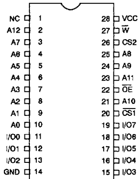
Pinout DIL/SO 28 pins (top view)
