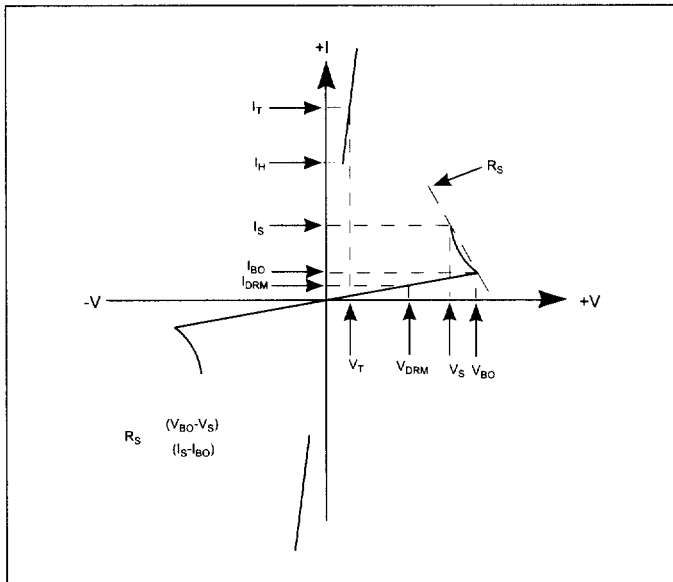
V-I Characteristics
