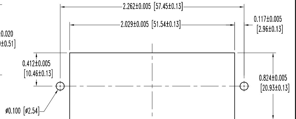
PANEL CUTOUT
