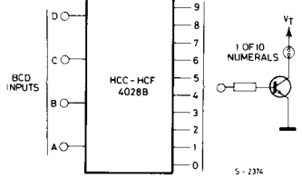
Fig. 4 - Neon readout (Nixie Tube) display application
