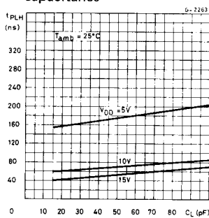
Typical propagation delay time as a function of load capacitance
