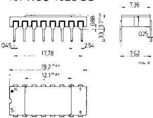
Dual in-line ceramic package for HCC 4028 BD
