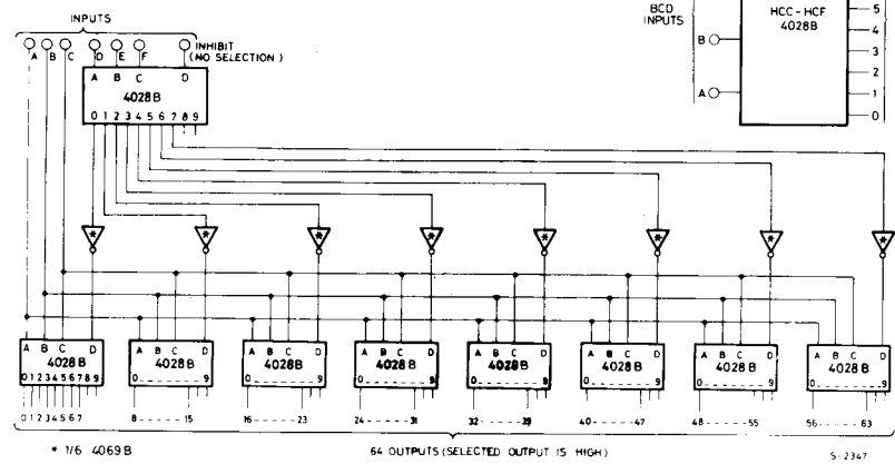
Fig. 3 - 6-bit binary to 1 of 64 address decoder
