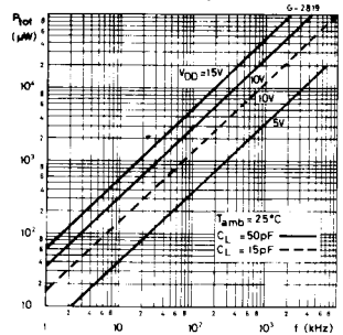
Typical dynamic power dissipation as a function of input frequency
