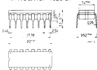
Dual in-line ceramic package for HCC/DCF 4028 BF
