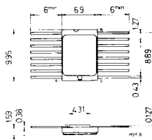
Ceramic flat package for HCC 4028 BK
