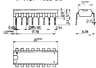
Dual in-line plastic package for HCF 4028 BE
