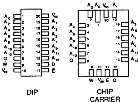
PIN CONFIGURATION
