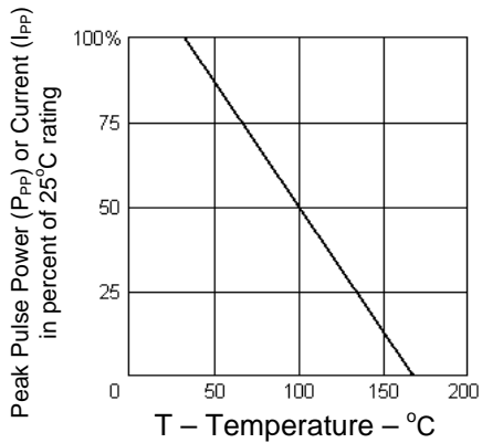
FIGURE 3 DERATING CURVE
