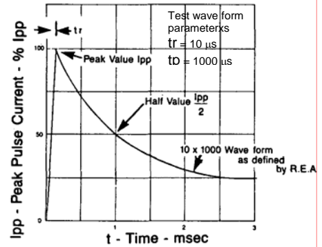
FIGURE 2 PULSE WAVEFORM
