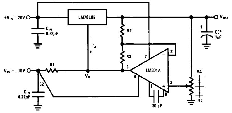
Variable Output Regulator 0.5V-18V
