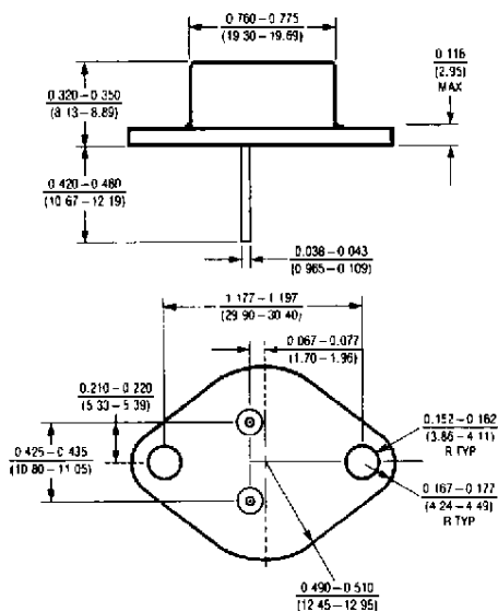
K Package TO-3 STEEL Metal Can
