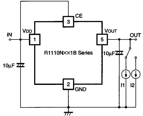
Test Circuit for Load Transient Response
