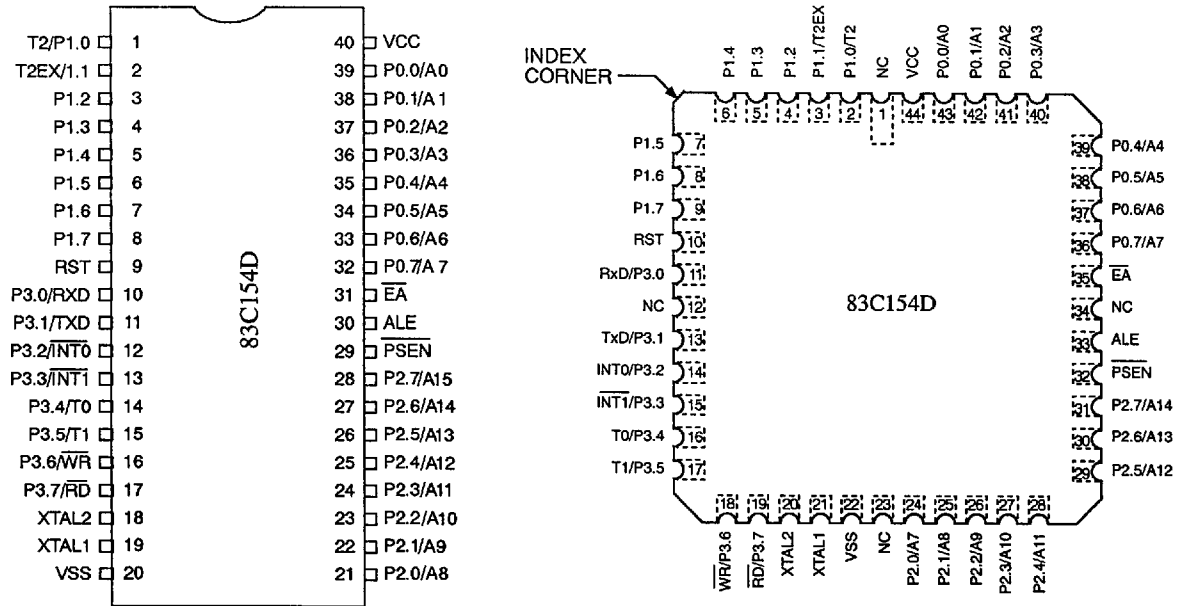
Figure 2. Pin Configuration
