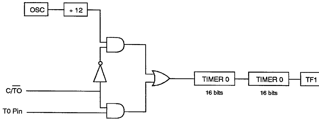
Figure 9. 32 Bit Timer/Counter.
