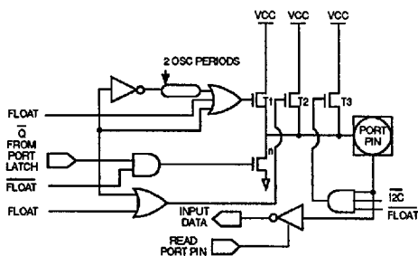
Figure 4. I/O Buffers in the 83C154D (Ports 1, 2, 3).
