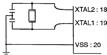
Figure 5. Crystal Oscillator.
