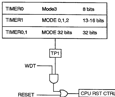
Figure 13. The Different Watchdog Configurations.
