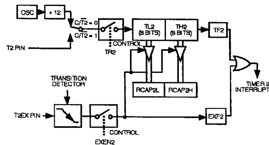
Figure 8. Timer in Auto-Reload Mode.
