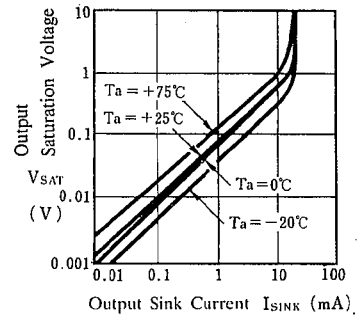
Output Saturation Voltage ( V^+ = 5V )
