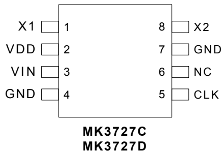
8-Pin (150 mil) SOIC
