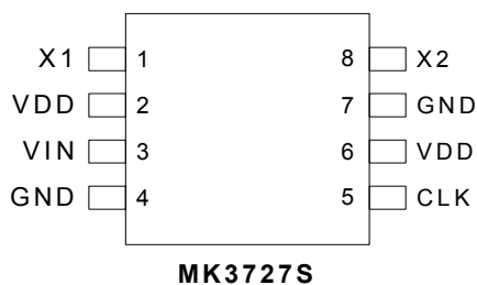
8-Pin (150 mil) SOIC
