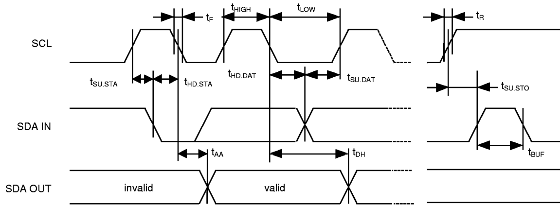
Figure 4 Bus Timing
