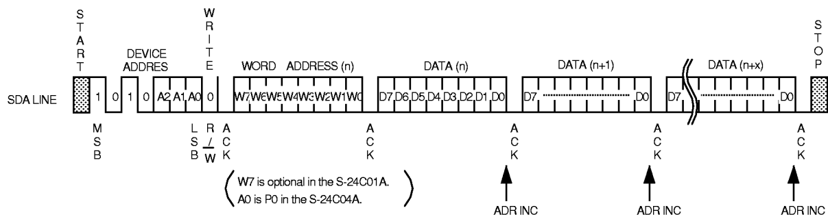
Figure 11 Page Write
