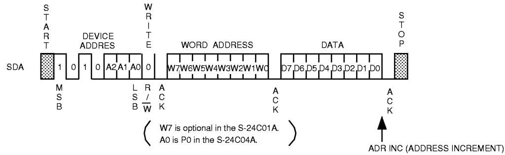
Figure 10 Byte Write
