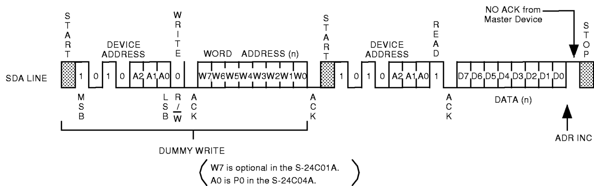
Figure 13 Random Read
