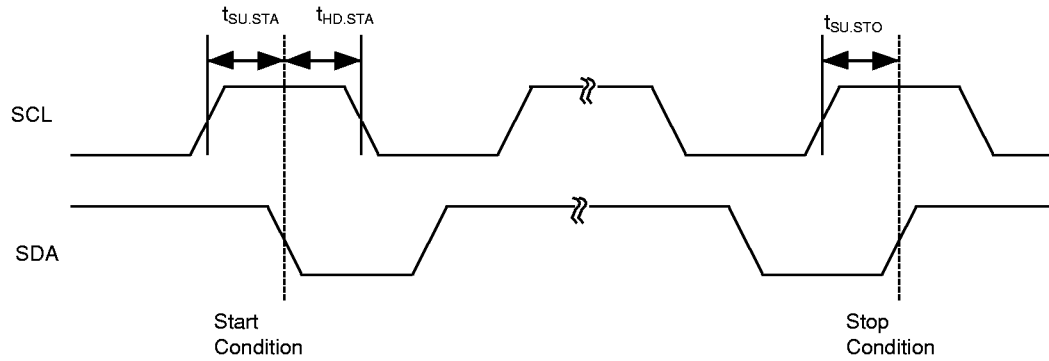
Figure 6 Start/Stop Conditions
