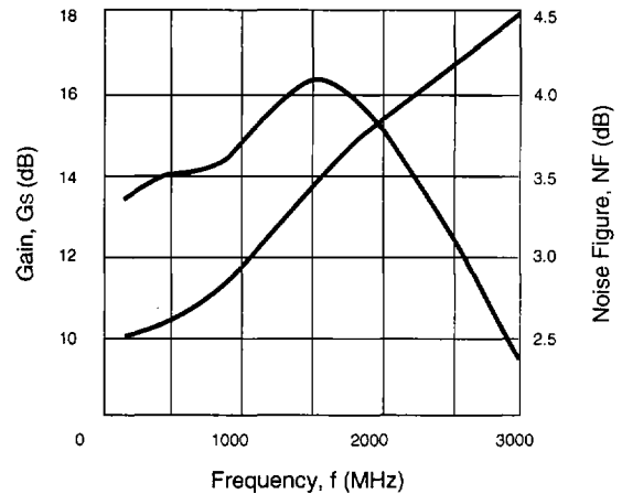
NOISE FIGURE AND GAIN vs. FREQUENCY V_{CC} = 3.0 V
