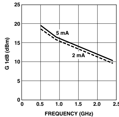
Figure 6. AT-30511 1 dB Compressed Gain vs. Frequency and Current at V_{\text{CE}} = 2.7\text{ V} .
