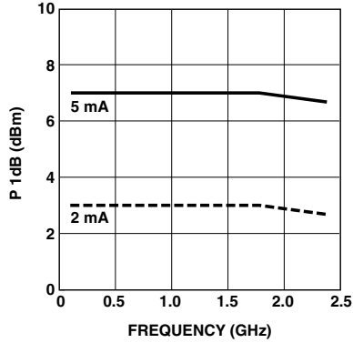
Figure 8. AT-30511 and AT-30533 Power at 1 dB Gain Compression vs. Frequency and Current at V_{CE} = 5\text{ V} .
