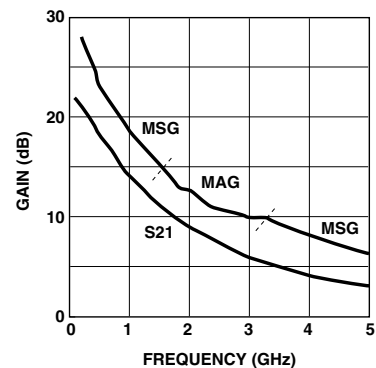
Figure 20. AT-30533 Gains vs. Frequency at V_{CE} = 2.7\text{ V} , I_C = 1\text{ mA} .
