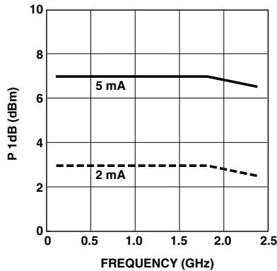
Figure 5. AT-30511 and AT-30533 Power at 1 dB Gain Compression vs. Frequency and Current at V_{\text{CE}} = 2.7\text{ V} .
