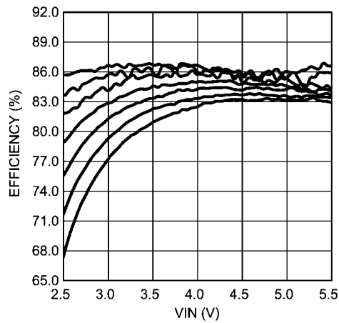
Efficiency vs VIN, Single String L = 22μH, 20mA/string, f SW = 1MHz Top to Bottom: 1x4, 1x5, 1x6, 1x7, 1x8, 1x9, 1x10 (LEDs)
