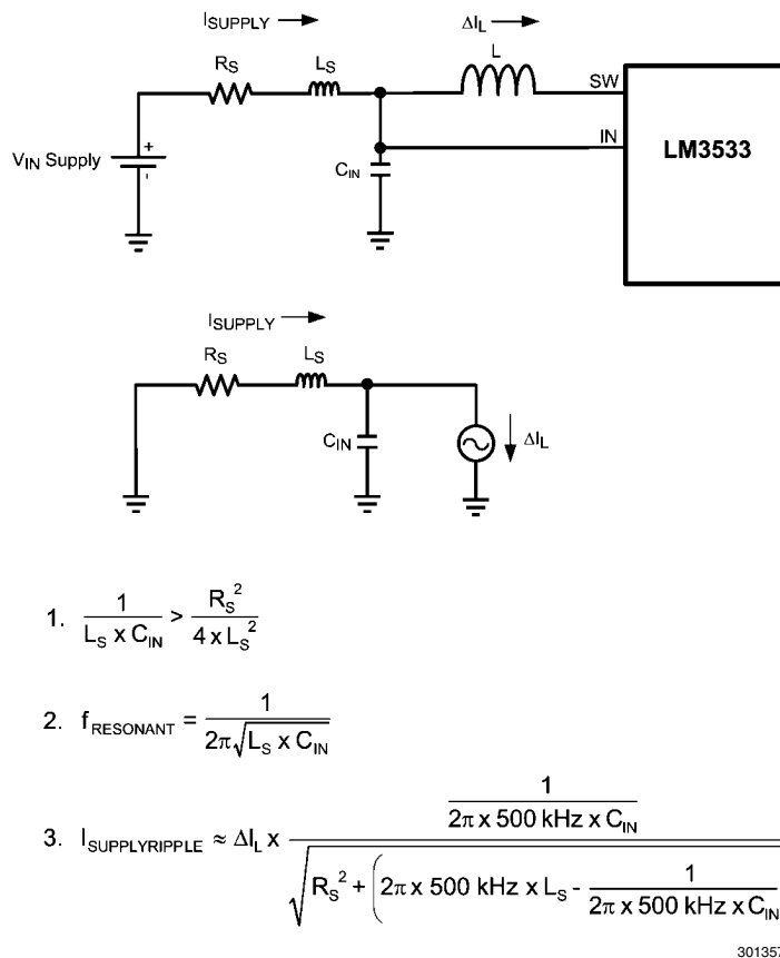
FIGURE 19. Input RLC Network
