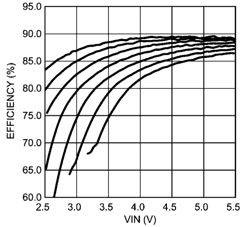
Efficiency vs VIN, Dual String L = 22μH, 20mA/string, f SW = 1MHz Top to Bottom: 2x4, 2x5, 2x6, 2x7, 2x8, 2x9, 2x10 (LEDs)
