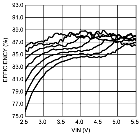
Efficiency vs VIN, Single String, L = 22μH, 20mA/string, f SW = 500kHz Top to Bottom: 1x4, 1x5, 1x6, 1x7, 1x8, 1x9, 1x10 (LEDs)
