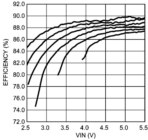
Efficiency vs VIN, Dual String, L = 22μH, 20mA/string, f SW = 500kHz Top to Bottom: 2x4, 2x5, 2x6, 2x7, 2x8, 2x9 (LEDs)
